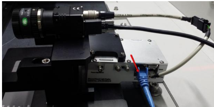
Figure 7 PSP 2 PROJECTOR PORT
