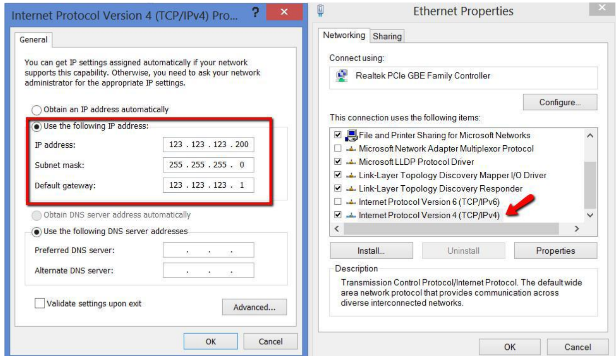
Figure 15 EBLE (PROJECTOR IP PORT) SETTING
