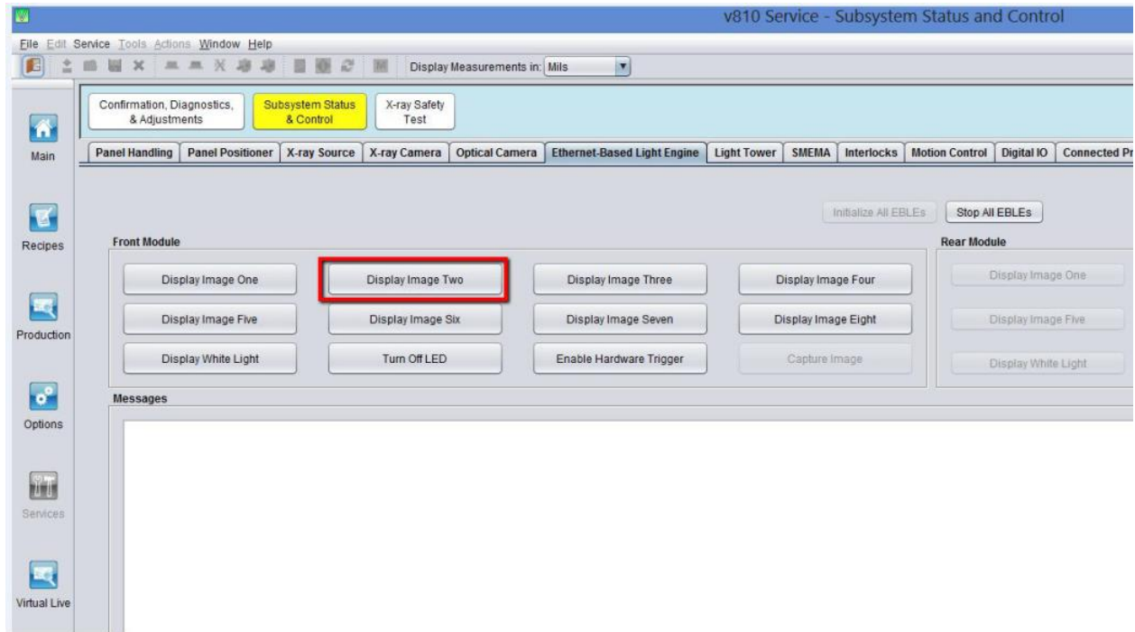
Figure 45 EBLE GUI
